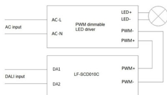
Wiring Diagram of DALI Dimming
