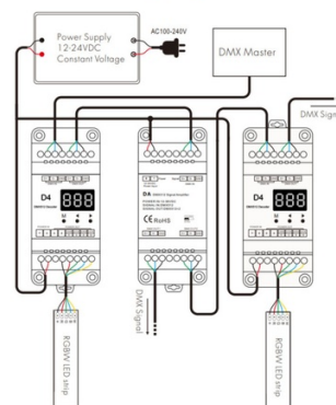
Wiring Diagram
