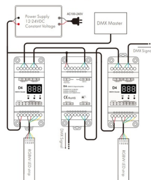
Wiring Diagram
