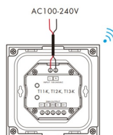
Wiring Diagram for rotary panel work as RF remote
