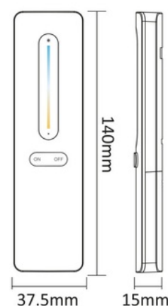
Remote
