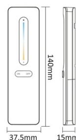
Remote
