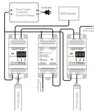
Wiring Diagram
