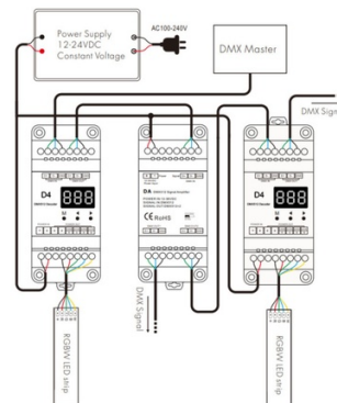
Wiring Diagram
