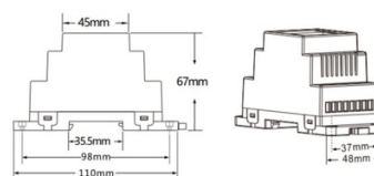
DIN Rail Mounting Size: TS-35/7.5 or TS-35/15
