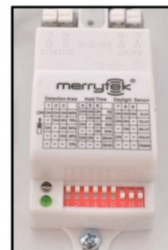
Area/Time/Daylight control Movement detector
